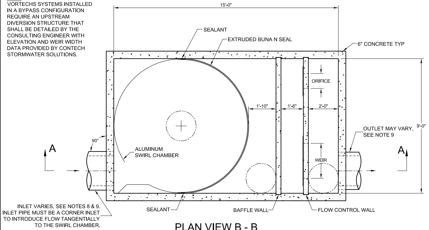
PLAN VIEW B - B
