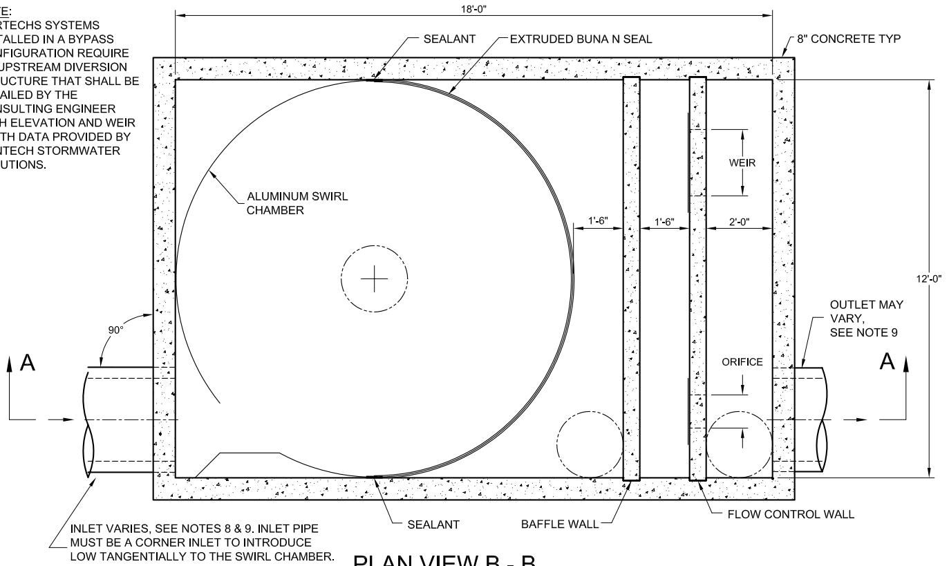
PLAN VIEW B - B
